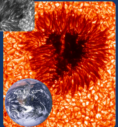
Sunspot & Earth comparison
